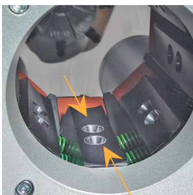
With the double pin connection it is possible to crimp on both sides of the s3 series machines.
