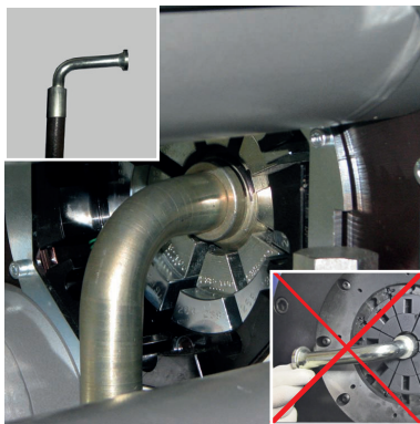
The S3 series allows to crimp short 90° Elbows fittings with a long drops. Impossible for other conventional machines.
