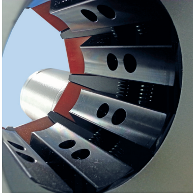
The S3 series is fitted with the clean slide bearing technology.
