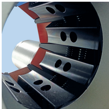
S6 series is fitted with the cleanliness greaseless slide bearing technology.
