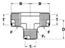
Union TEE Male ORFS
