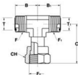
Swivel branch tee Male ORFS - swivel nut ORFS
