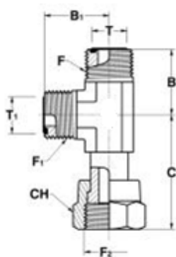
Swivel run tee Male ORFS - swivel nut ORFS
